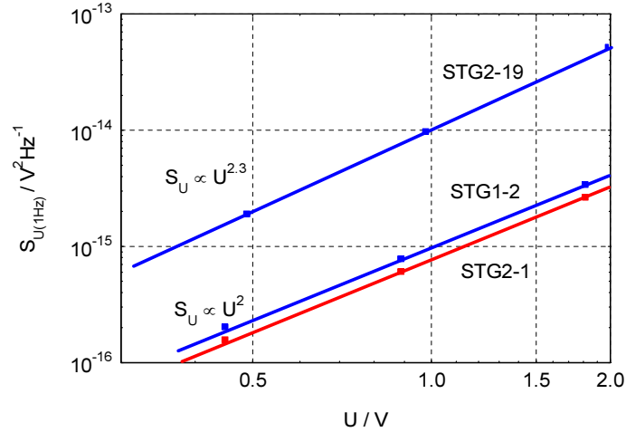
Fig. 9. The noise spectral density S_{U(1\text{Hz})} at f=1 Hz vs. bias voltage U for samples STG1-2, STG2-1 and STG2-19 after subtraction of measuring set-up background noise measured at a temperature of T = 24^\circ\text{C} .
