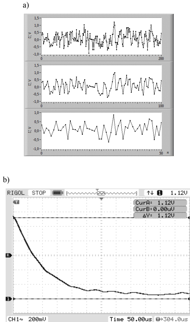
Fig. 3. Experimental characteristics: a) fragments of signal realizations x(i\Delta t_p) from sampling intervals \Delta t_p equal subsequently to: \Delta t_{p1} = 50 \mu\text{s} , \Delta t_{p2} = 100 \mu\text{s} , and \Delta t_{p3} = 200 \mu\text{s} ; b) function of the conditional mean value of the analyzed signal \bar{x}_w = f(k\Delta t_{p1}) .
