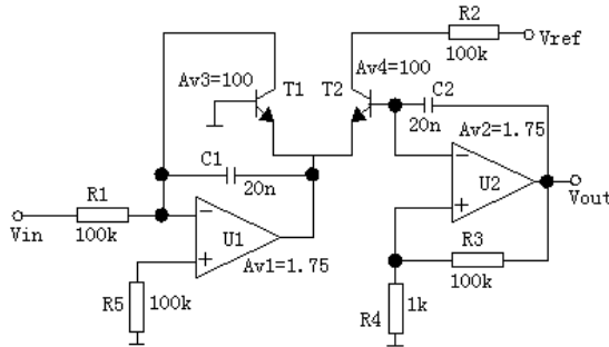
Fig. 10. Logarithm amplitude circuit in simulation 2.
