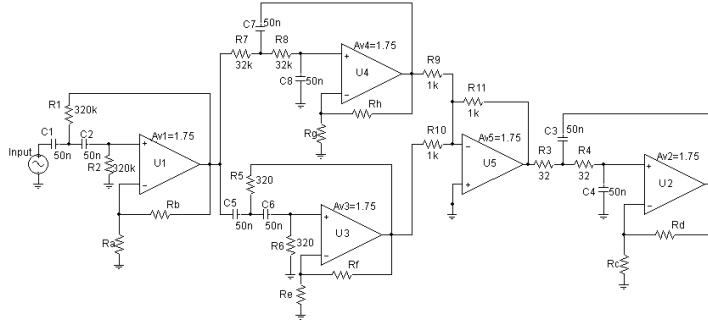
Fig. 3. Simulation 1- The band-pass filter circuit.
