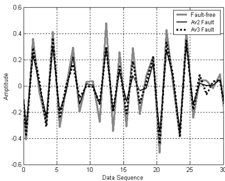
Fig. 4. Linear Volterra series in full band.
