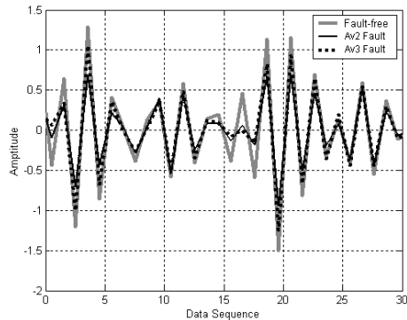
Fig. 5. Quadratic Volterra series in fullband.
