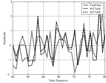
Fig. 7. Quadratic Volterra series in feature subband.
