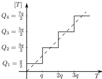
Fig. 1. A quantizer (quantization transfer function).
