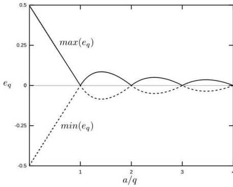
Fig 9. Minimum and maximum values of quantization error as a function of width of rectangular distribution of noise.
