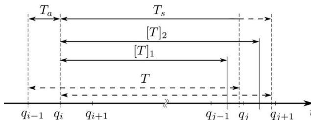
Fig. 3. Asynchronous measurement of time-interval T .
