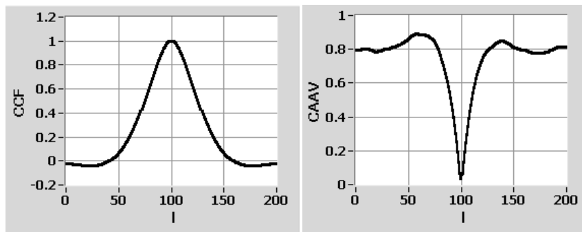
Fig. 3. CCF and CAAV obtained from the simulation.
