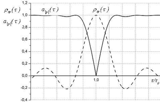
Fig. 1. Examples of normalized CCF and CAAV functions.
