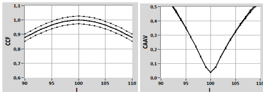
Fig. 4. CCF and CAAV for \sigma_z = 0 .
