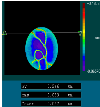
Fig. 6. Analysis of the cracked surface by a laser interferometer.
