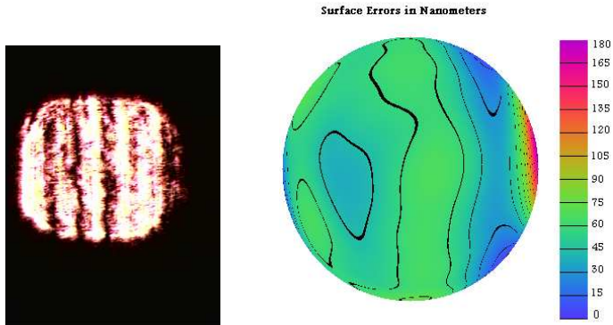
Fig. 2. Analysis of surface flatness using digital holography.
