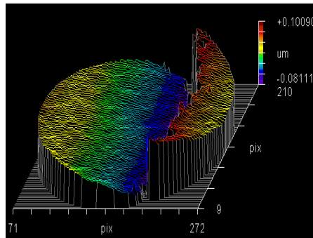
Fig. 3. Analysis of surface flatness by laser interferometer.
