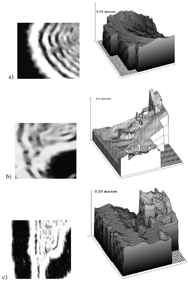
Fig. 5. Surface variations at a) crack propagation; b) crack end; c) crack split.
