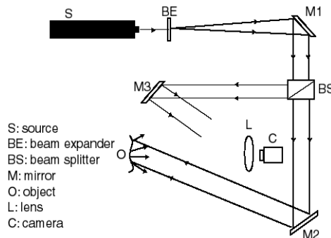
Fig. 1. The scheme of the holographic technique.
