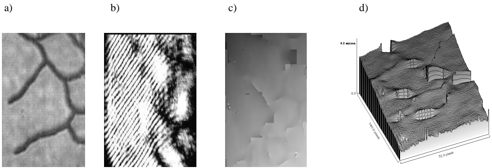
Fig. 4. a) Crack on a steel object; b) the recorded hologram; c) the unwrapped phase; d) crack effect on surface plane.
