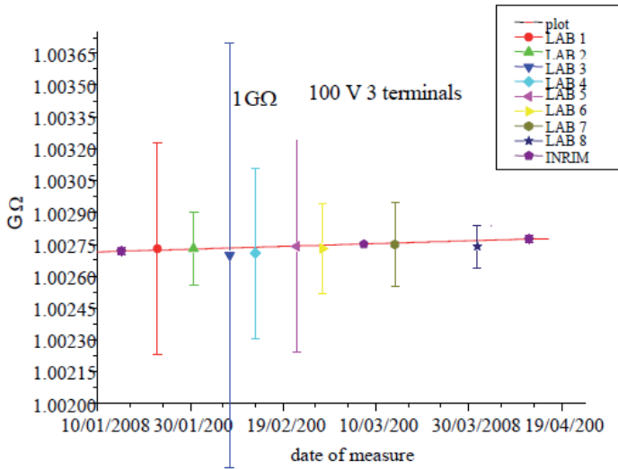
Fig. 9. Results for the 1 GΩ at 3 terminals at 100 V.
