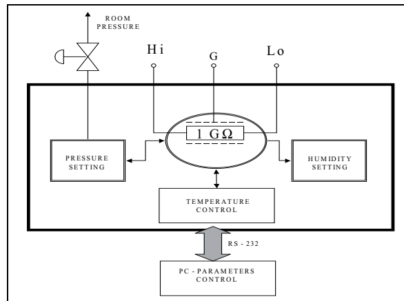
Fig. 2 . Block diagram of the 1 GΩ resistor.
