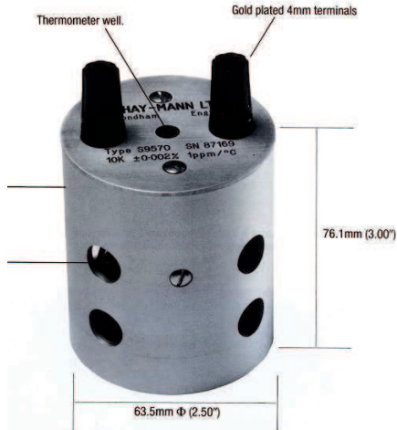
Fig. 1. The Vishay-Mann 10 MΩ.
