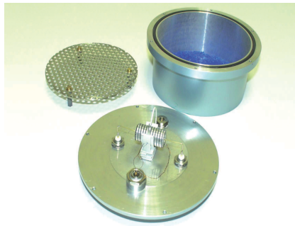
Fig. 4. The hermetic container of the resistor: is also visible the grid under which there is the silica gel for humidity control.
