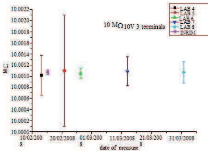
Fig. 7. Results for the 10 MΩ at 3 terminals at 10 V.
